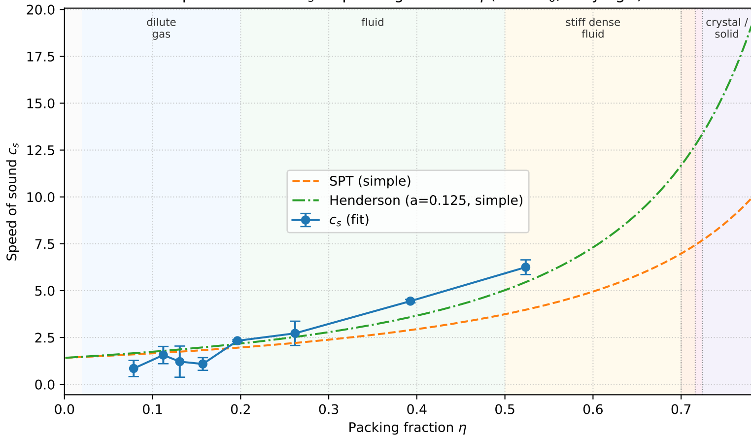
Speed of sound c_s vs packing fraction \eta (fixed L_0 , varying r )
